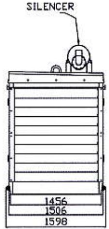
VIEW FROM ALTERNATOR SIDE
